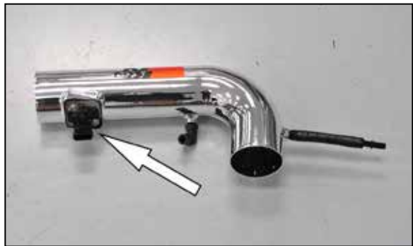
23. Install the mass air assembly into the K&N® intake tube as shown.
