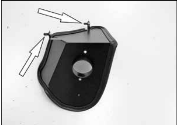
14. Install the two provided mounting posts onto the heat shield using the provided hardware.
