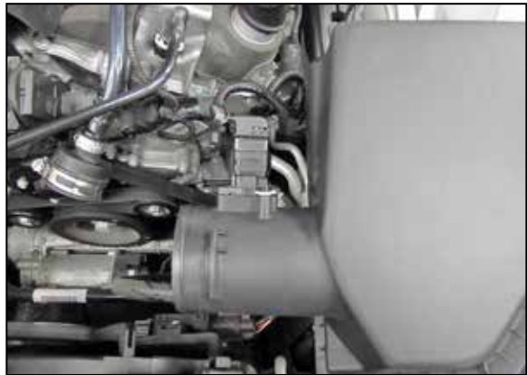
9. Disconnect the mass air sensor electrical connection.
