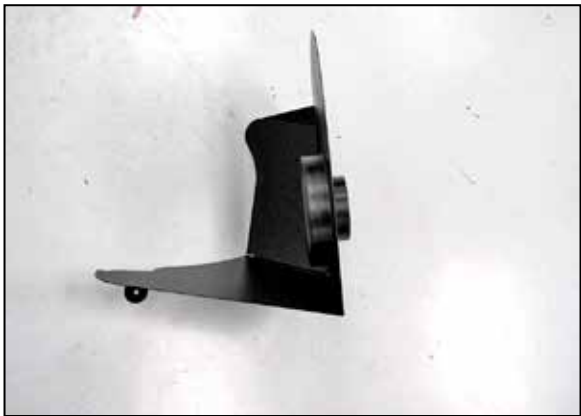
12. Install the filter adapter into the heat shield and secure with the provided hardware.
